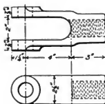
Figs. 4271-4272. Reach Rod Jaw.
